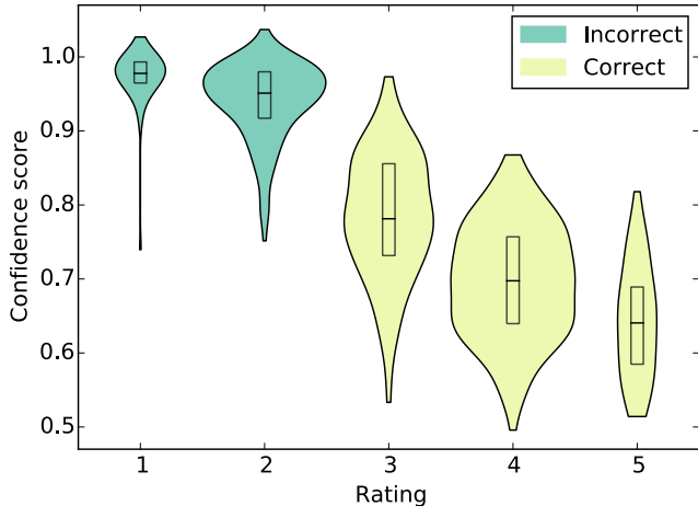
Fig. 1. Violin plot (box plot with rotated kernel density estimates) showing the distribution of confidence scores for each rating in our qualitative evaluation. A smaller confidence score indicates a more successful alignment. The area of each violin corresponds to the number of pairs which had a given rating. Box plots in each violin show the median and upper and lower quartiles.
